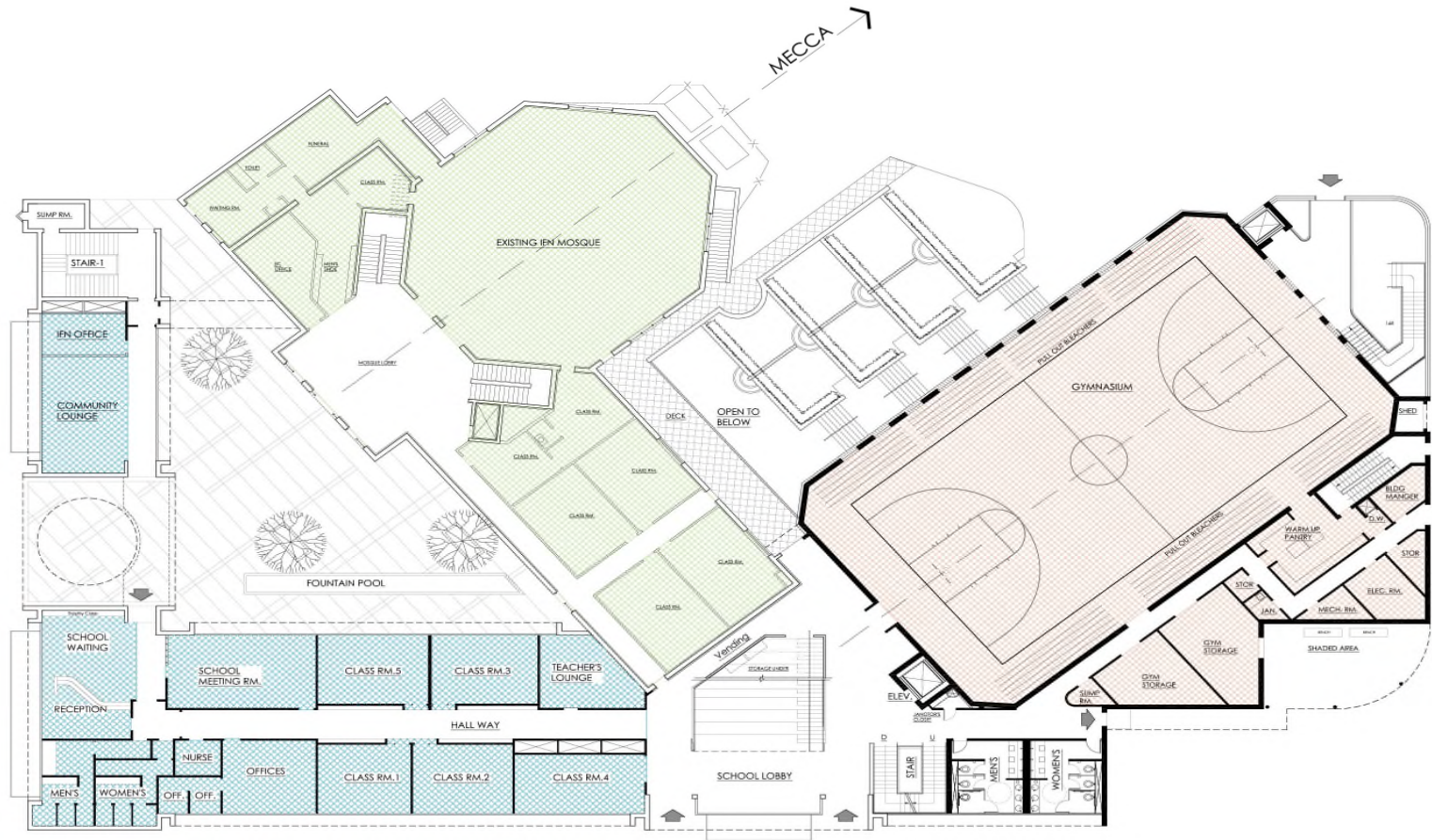
5 FIRST FLOOR PLAN
